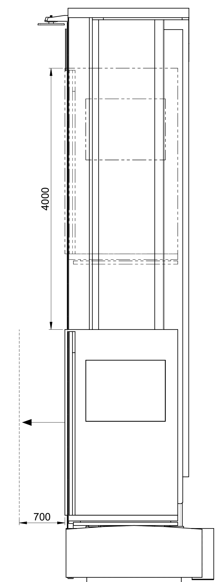
CORSE PEDANA OPERATORE OPERATOR PLATFORM'S STROKES
